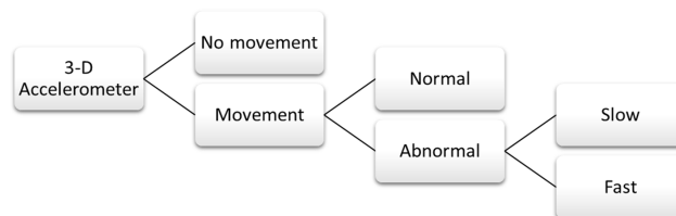
Fig. 4. Decision tree.
